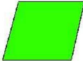
parallelogram
